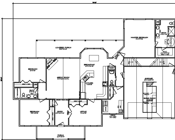
1 FIRST FLOOR PLAN A-3
