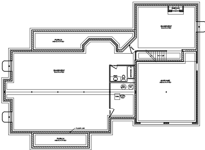
1 FOUNDATION PLAN A-2
